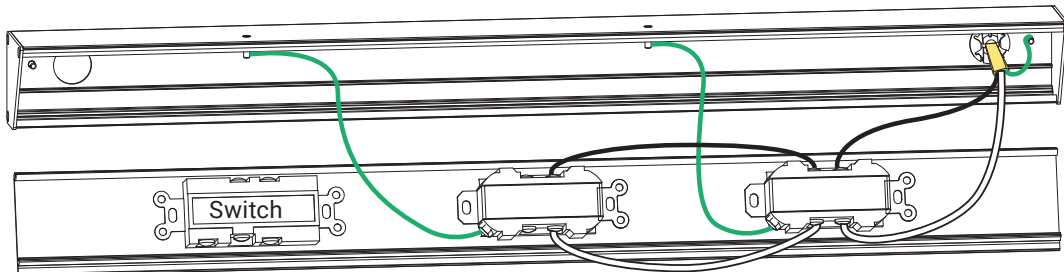
TRS Series Wiring Diagram
