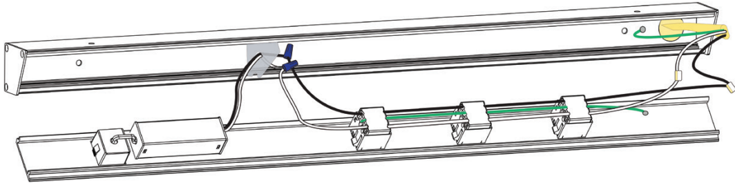
APT-USB Series Wiring Diagram
